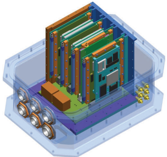
Figure 3. TacSat-1 Copperfield-2 CompactPCI Cardset and Chassis
