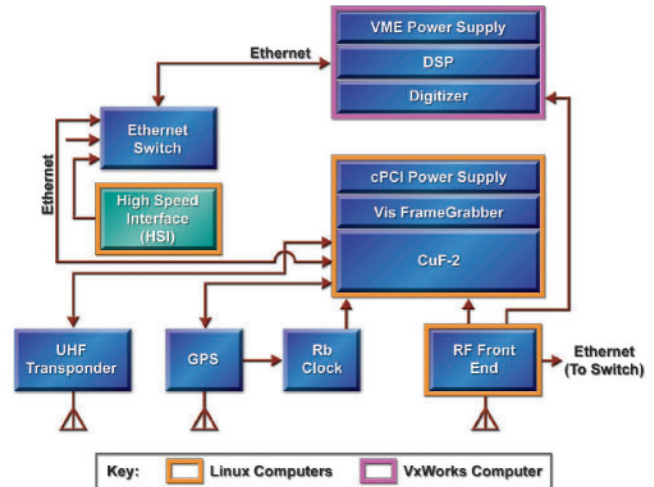
Figure 2. TacSat-1 Copperfield-2 Payload Block Diagram
