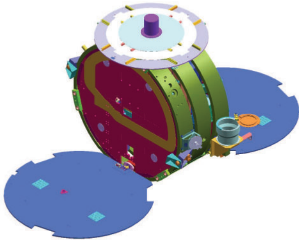
Figure 1. TacSat-1 Spacecraft, Solar Arrays Deployed, Nadir (Earth-Facing) Side Facing Up
