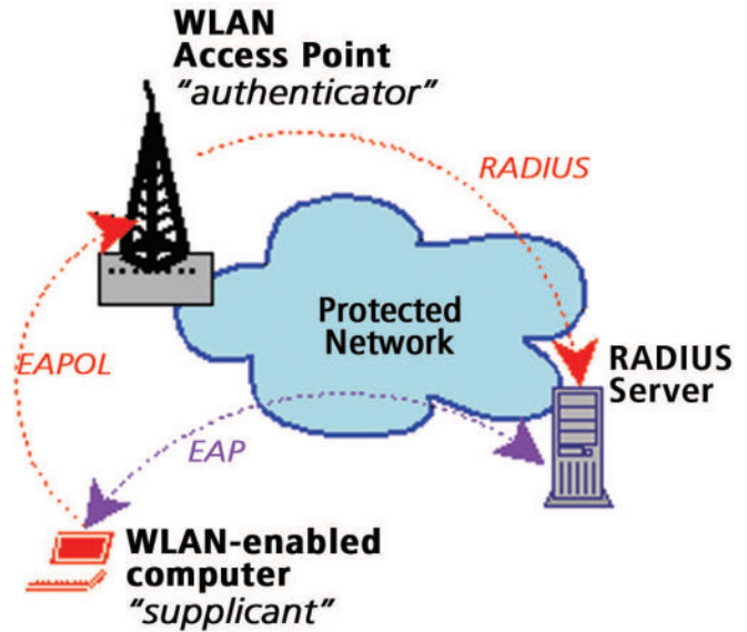
Figure 1. WPA Topology
