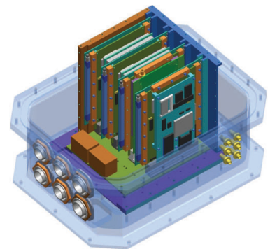
This sensor system started life on an unmanned airplane but became part of the TacSat-1 satellite project (page 40).
