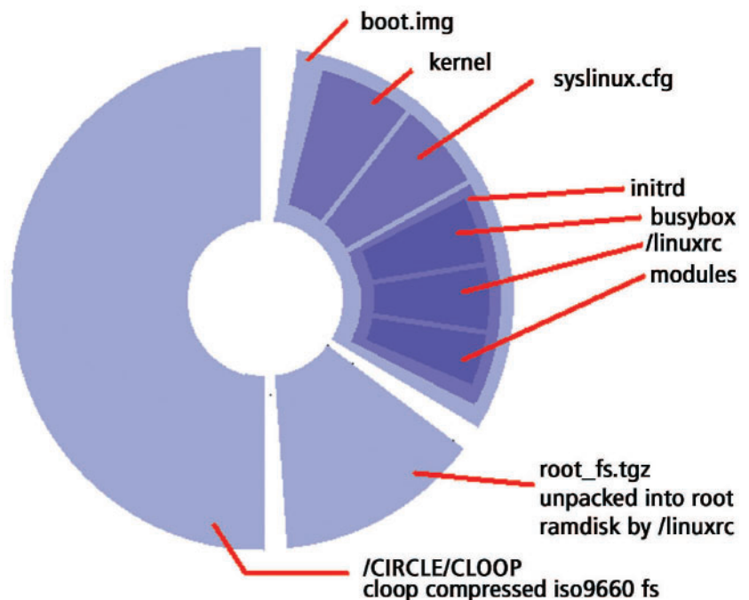
Figure 1. Wheels within wheels: the finished CD nests filesystem images inside filesystem images inside filesystem images.
